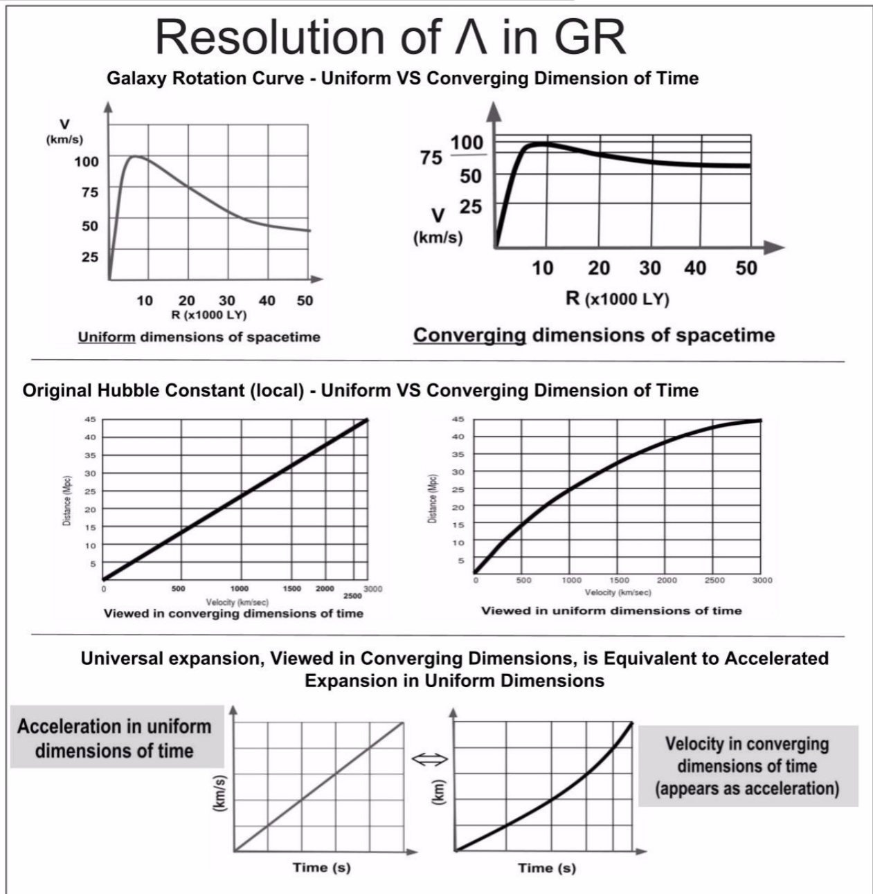
FIG. 6: converging dimensional space in GR
