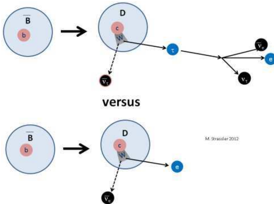
Fig. 1: Lepton universality predicts that the two processes shown — the decay of a B meson to a D meson, an anti-neutrino and a tau or electron, involving the weak nuclear force via a W 'virtual particle' — should differ in probability only through the calculable effect of the tau lepton's mass, which makes the tau decay a bit less likely. The tau will rapidly decay, sometimes to an electron or muon, along with an undetectable neutrino and anti-neutrino. The D meson will also rapidly decay to other particles (not shown); these must all be experimentally detected in order to know a D meson was present. Only the bottom and charm quarks in the mesons are shown, but the mesons also contain an up and down anti-quark, along with many gluons and quark-antiquark pairs. [13]
