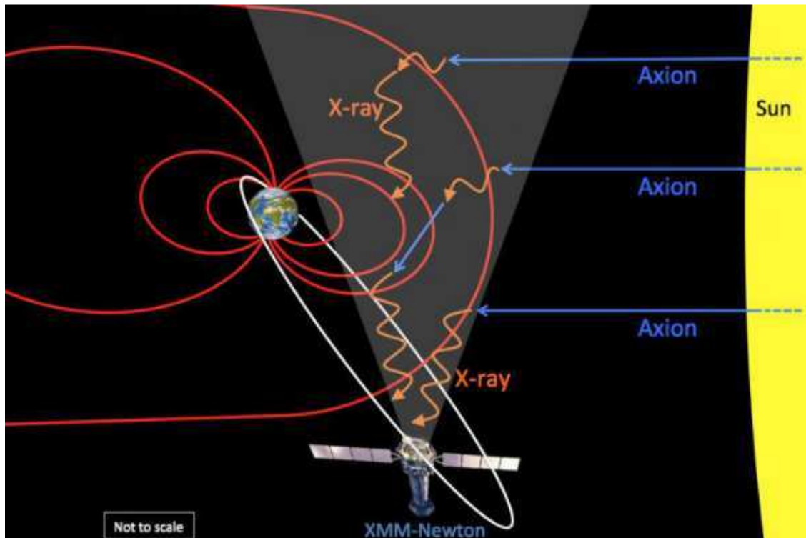
A sketch (not to scale) shows axions (blue) streaming out of the Sun and then converting into X-rays (orange) in the Earth's magnetic field (red). The X-rays are then detected by the XMM-Newton observatory. [13]
